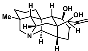
Kobusine
