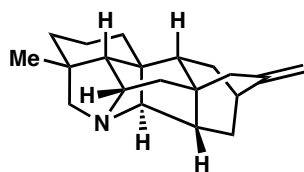
Hetisine Core
