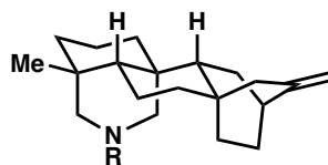
Atisane Core
