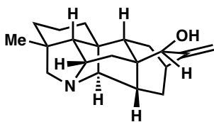
Nominine
